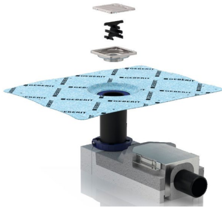
Fig. 3 Geberit gulvsluk for rist – Slukrist Standard Figur: Geberit AS
