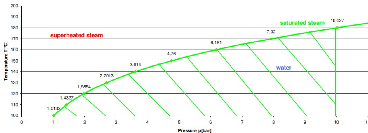
Vapor-Pressure-Table Temperature 100 °C - 200 °C
