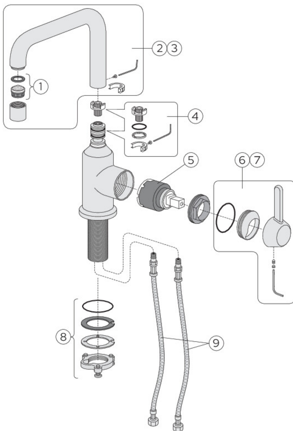
ExplodedView Ducentic_kitchen_1-hole (Rev I. 2024-11-05)
