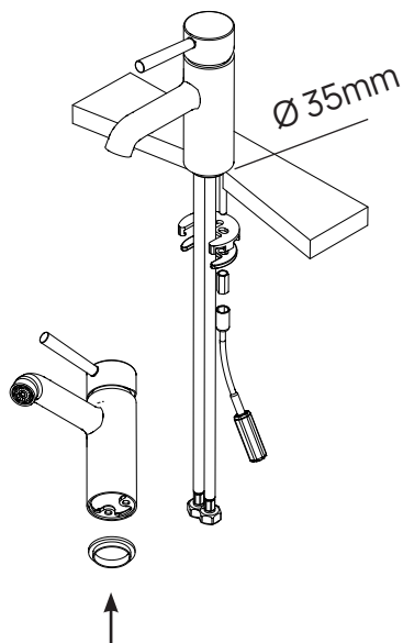
Montering uten base plate
