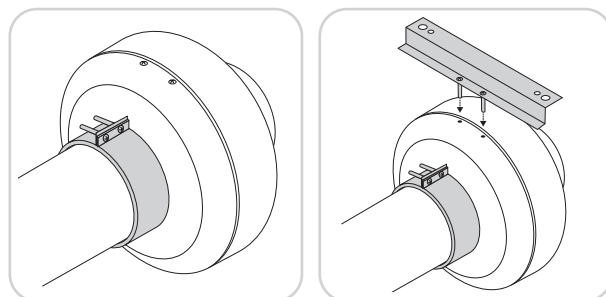
Installation with mounting clip and bracket (accessories).
