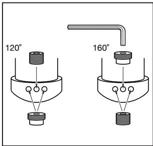
Figure 3A On faucets of the type Rin and Sk the swing radius can be set between 120° or 160° by repositioning the three locking plugs as shown in Figure 3A . The plugs are screwed in and out using an Allen key.
