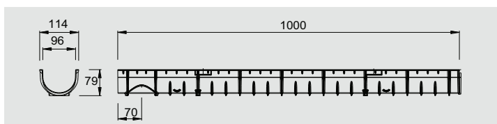
Ränna Meahome Plus
